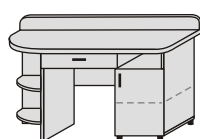
SG-35 150/60/75+10
